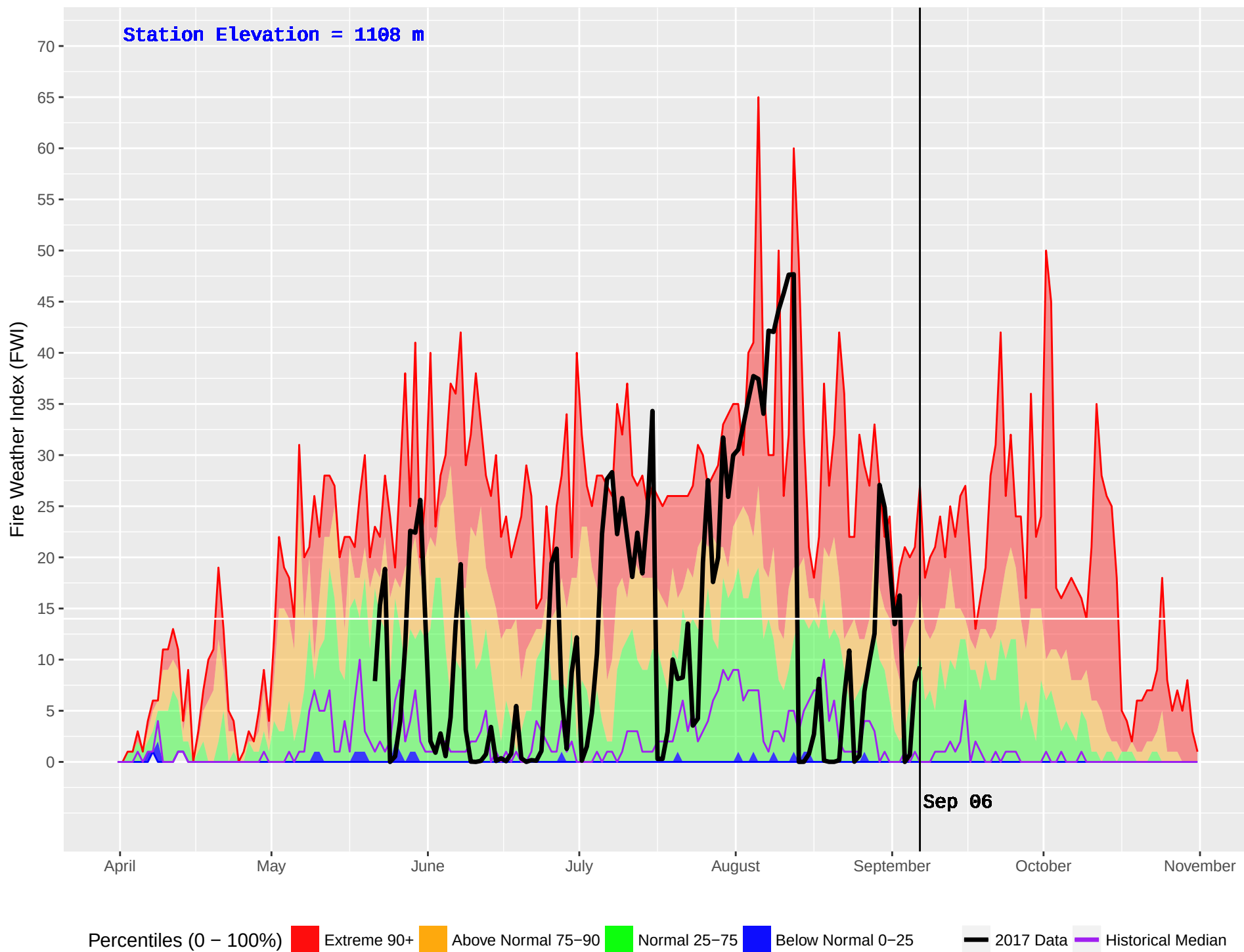
MATHEW (263) : Historical (1987–2016) and Current (2017) Noon Fire Weather Index (FWI)
